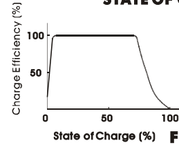
Figure22. CHARGING EFFICIENCY VS STATE OF CHARGE
