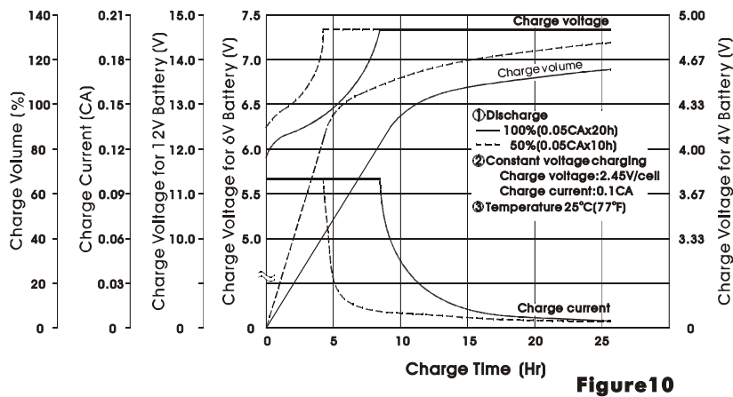
Figure10. BATTERY CHARGING CHARACTERISTICS (Typical example of the charge characteristics for the cycle use)
