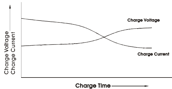
Figure 13. CHARGING CHARACTERISTICS OF A TAPER CHARGER
